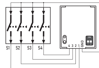
Button connection
