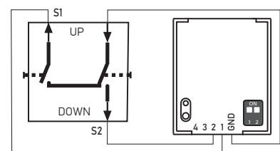
Blind switch connection
