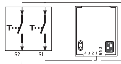
Switch connection
